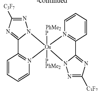
Os(hptz) 2 (PPhMe 2 ) 2
