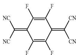
&lt;F4-TCNQ&gt;
