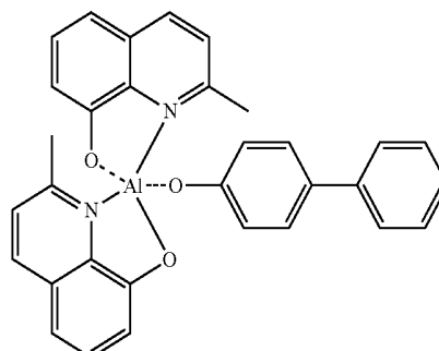
BAIq
