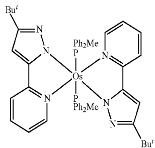
Os(bppz) 2 (PPh 3 ) 2
